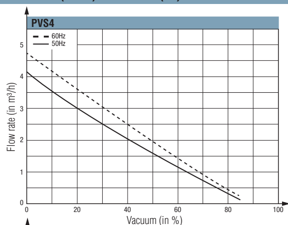
Flow rate (m³/h) / Vacuum (%)
